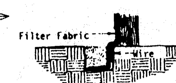
CONSTRUCTION OF A SILT FENCE
